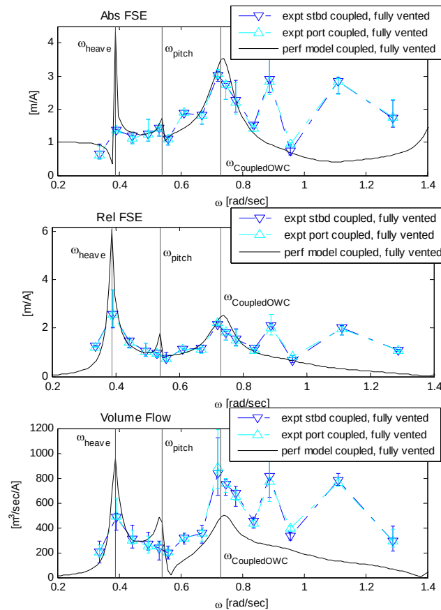
Figure 1-15: Experimental verification of \omega_{copuledOWC} through RAOs of absolute FSE, relative FSE, and volume flow for a fully vented BBDB.
