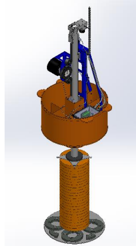
Figure 2 WEC Archetype II - LUPA (Point absorber wave energy converter type).
