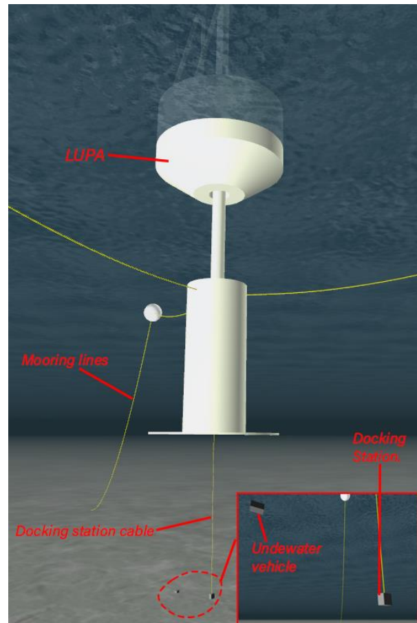
Figure 6 LUPA WEC-AUV coupled model.
