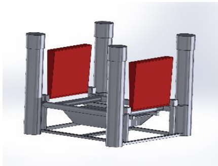
Figure 1 WEC Archetype I - FOSWEC2 (Oscillating surge wave energy converter type).
