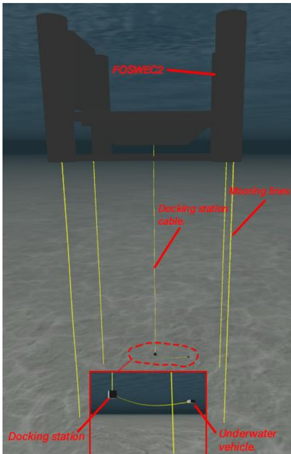
Figure 5 FOSWEC2 WEC-AUV coupled model.
