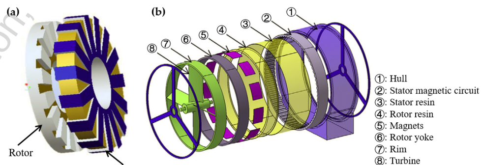
Figure 8. Schematic of DDPM synchronous generators: (a) a single-stator single-rotor axial-flux DDPM synchronous generator [113] and (b) a radial-flux DDPM synchronous generator [117].
