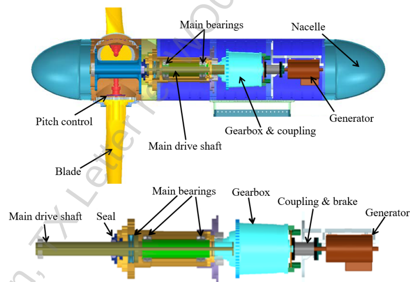
Figure 1. Schematic of a power conversion chain of the TCEC [47].
